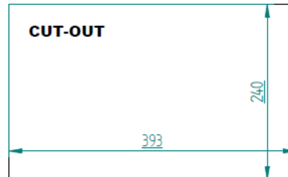
STANDARD FRONT PANEL VERSION
